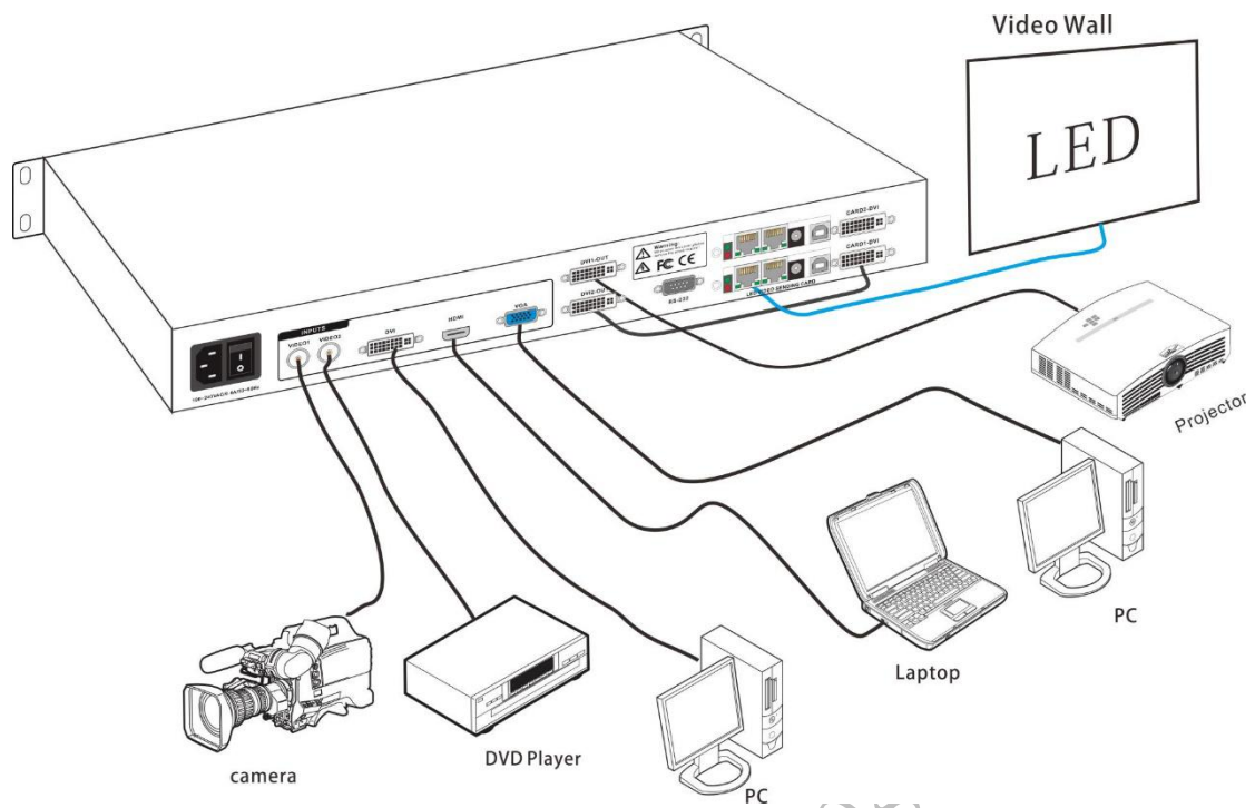
Connection diagram
